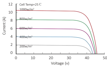
Current-Voltage Curve (RS6K-330M)
